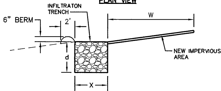
SECTION VIEW
